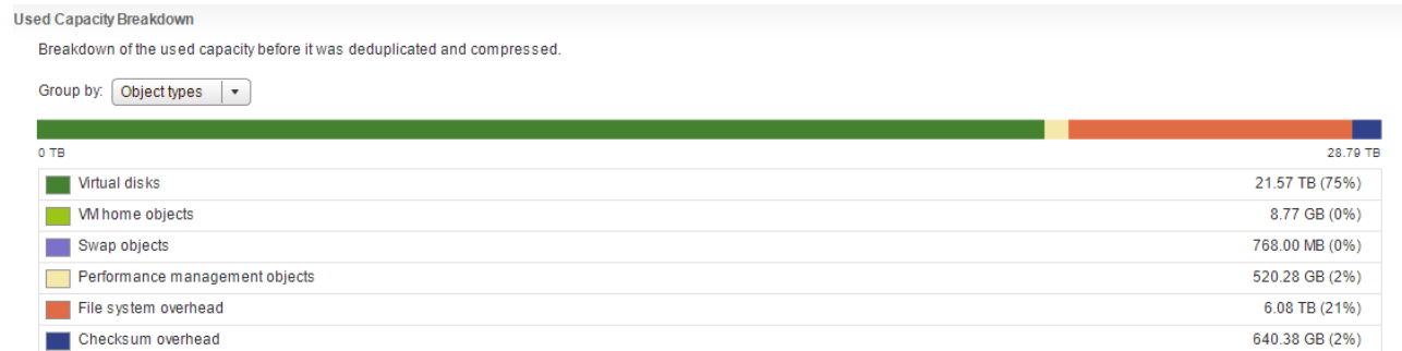
Figure 18: Capacity Test Object Type Breakdown
