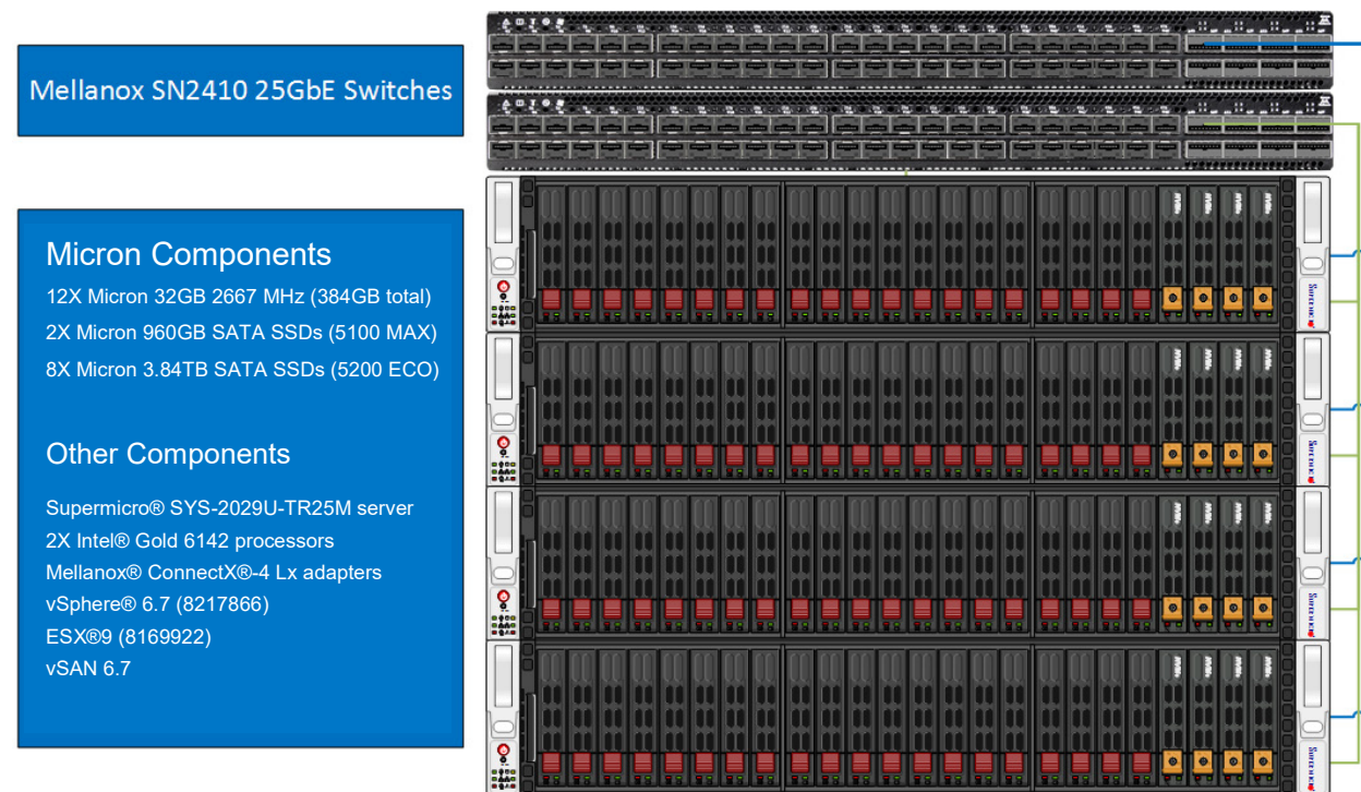
Figure 2: Hardware Components
